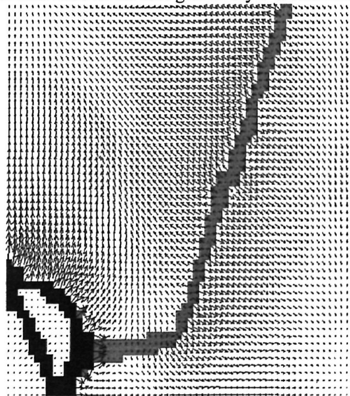
Figure 4: Direction of flow in the first ground layer around Ismailia Canal
