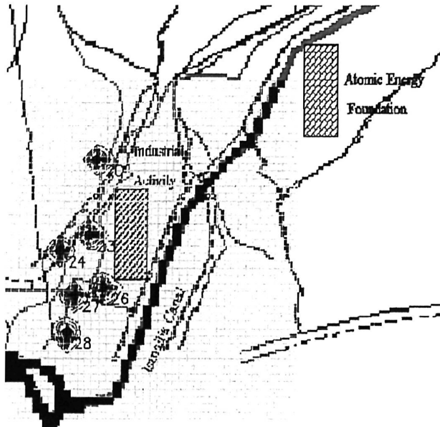
Figure 5: Cd distribution around ground wells after 30 days
