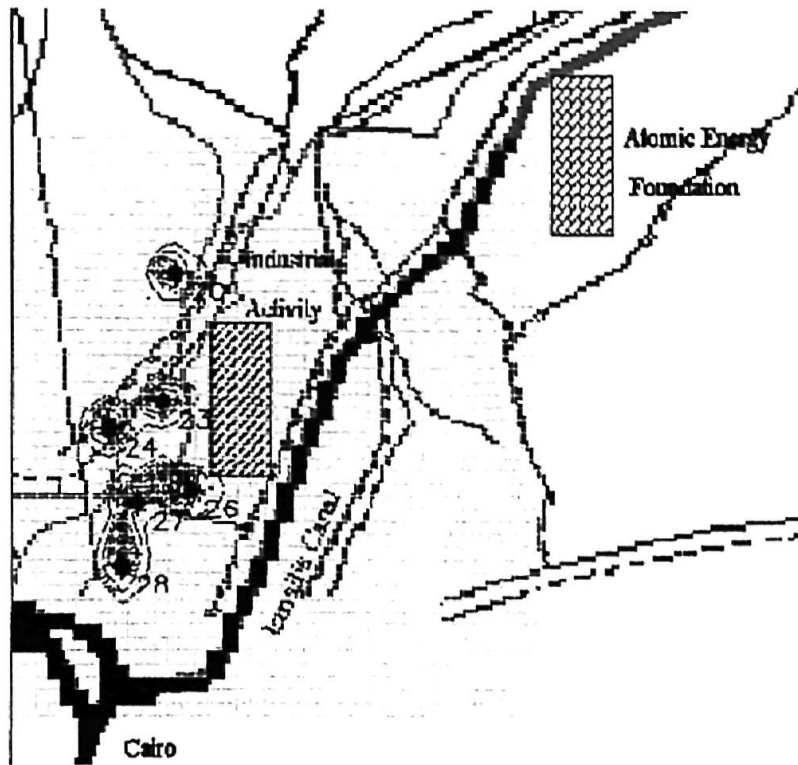
Figure 6: Cd distribution around ground wells after 6 months
