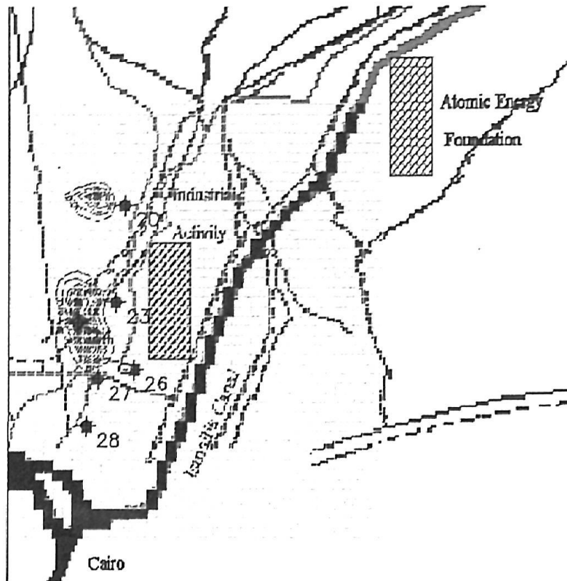
Figure 8: Cd distribution around ground wells after three years
