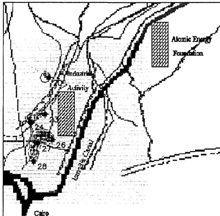
Figure 7: Cd distribution around ground wells after one year
